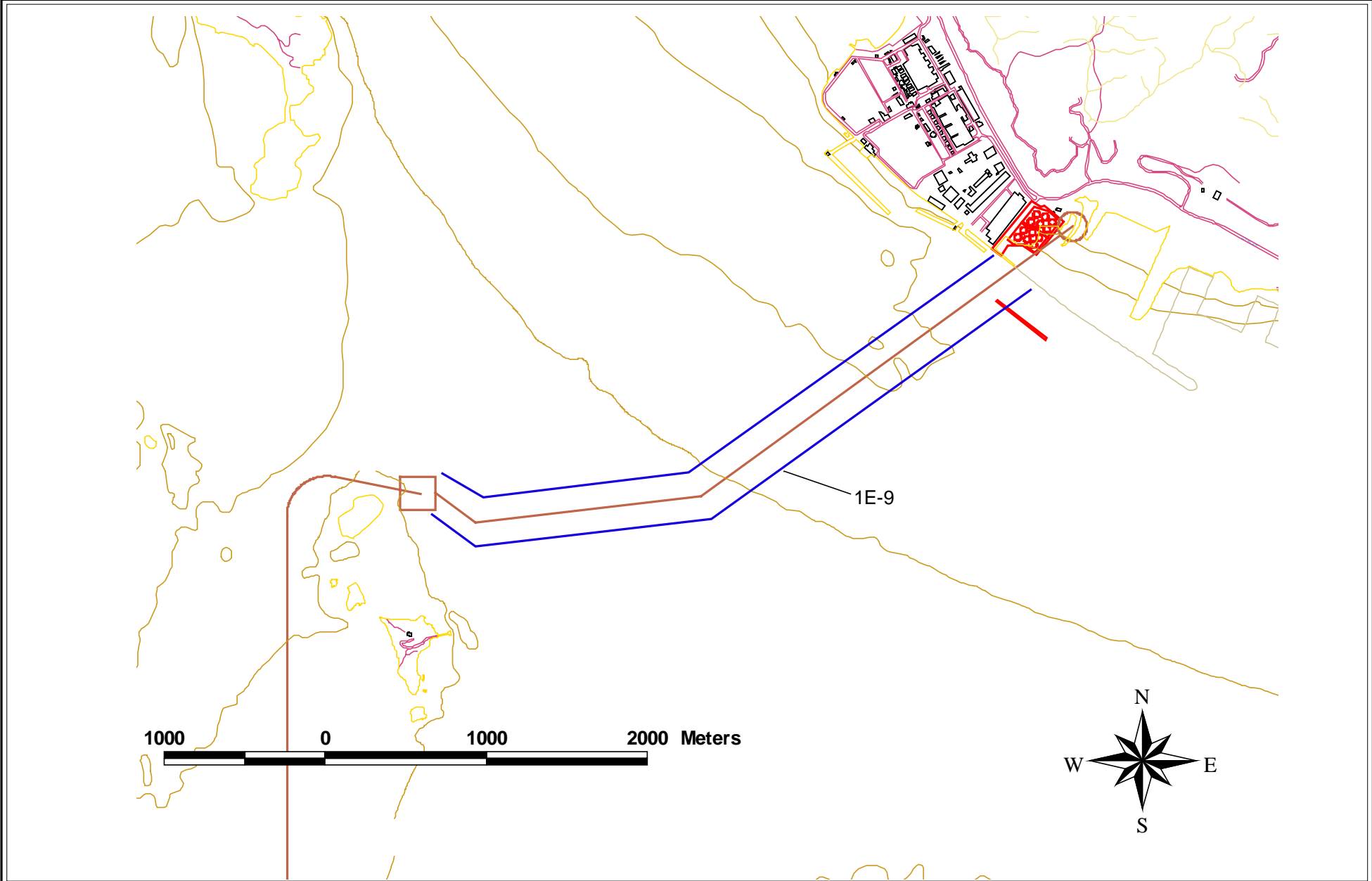
INDIVIDUAL RISK FOR SUBMARINE PIPELINE
